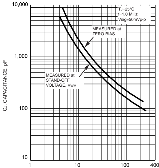
FIG. 5 - TYPICAL JUNCTION CAPACITANCE BIDIRECTIONAL
