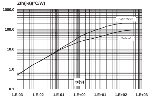
Fig. 4: Variation of thermal impedance junction to ambient versus pulse duration.
