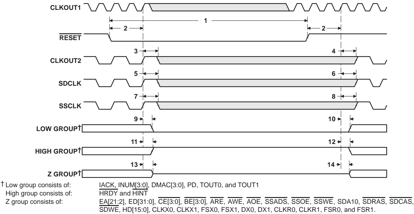
Figure 26. Reset Timing
