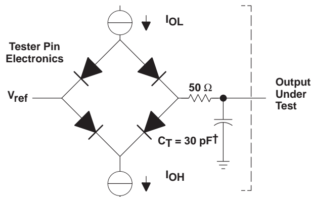
Figure 7. TTL-Level Outputs
