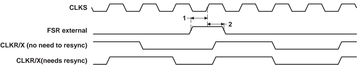
Figure 33. FSR Timing When GSYNC = 1
