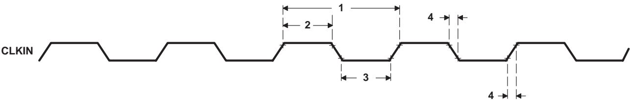
Figure 9. CLKIN Timings
