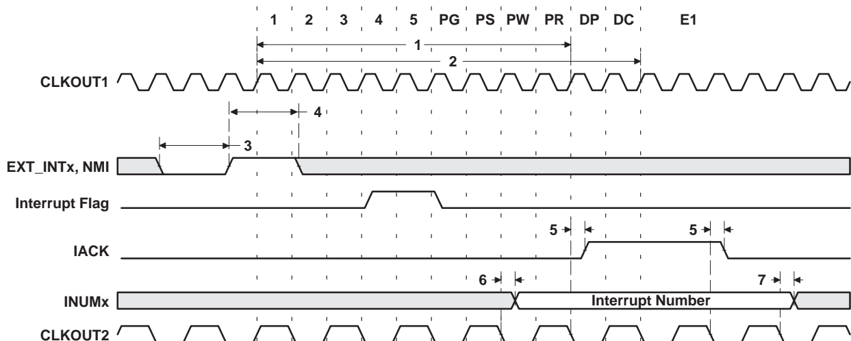
Figure 27. Interrupt Timing
