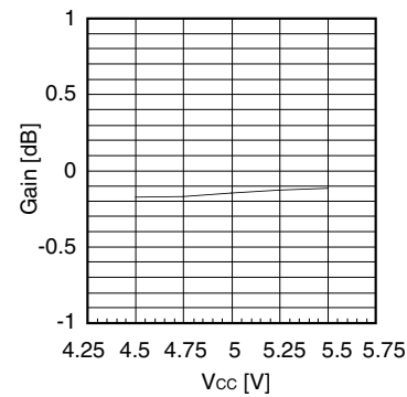
Figure 28. Gain vs. V_{CC} (0dB)
