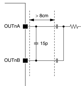
Figure 7. Oscillation prevention capacitor connection
