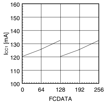
Figure 25. I_{CC1} vs. FCDATA (6dB)
