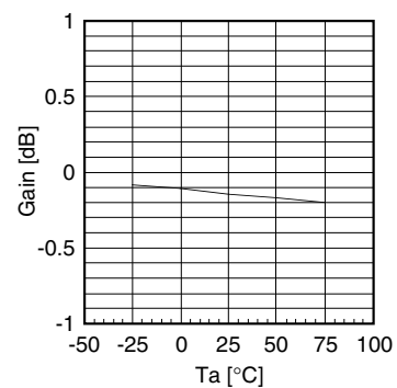
Figure 29. Gain vs. T_a (0dB)
