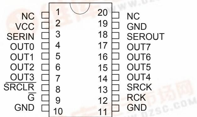
SM6B595F 20 PIN SOP
