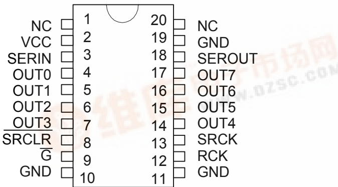
SM6B595P 20 PIN DIP
