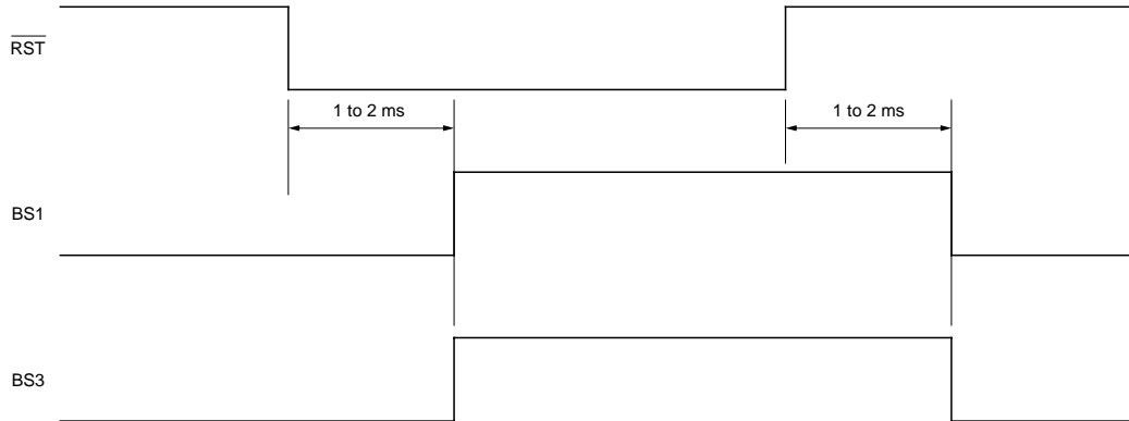
Figure 10. Extended reset timing
