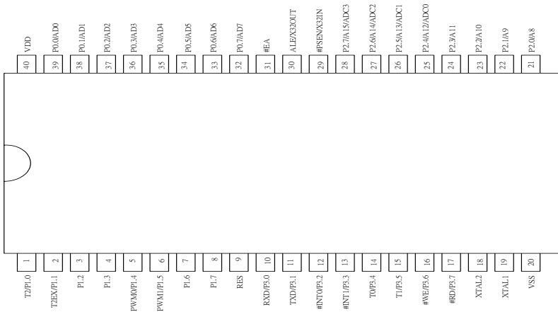
Figure 3 40L PDIP Package
