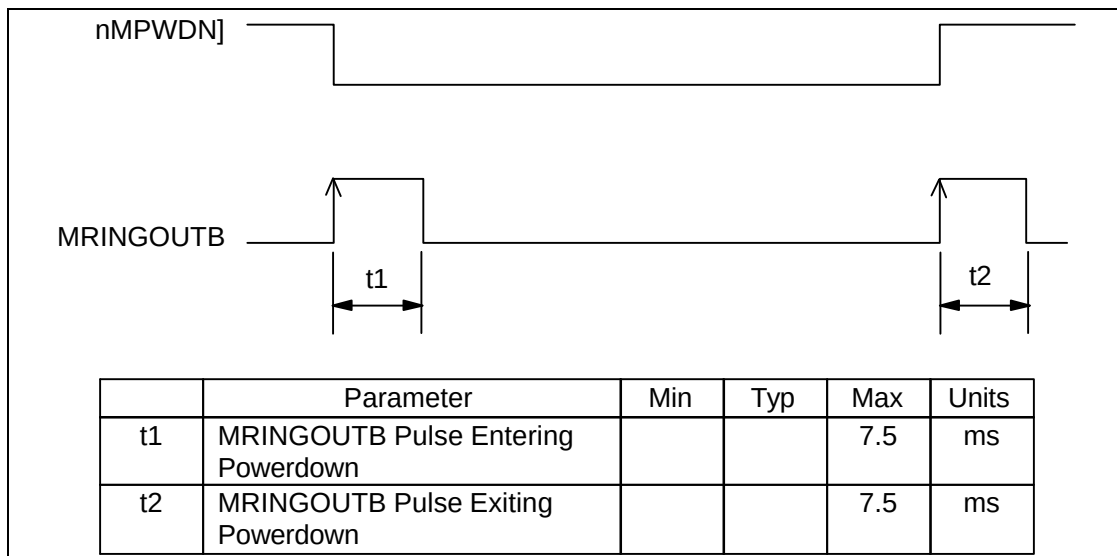
FIGURE 26 - RINGOUT FOR L39/C39 ROCKWELL MODEMS ENTERING/EXITING POWERDOWN
