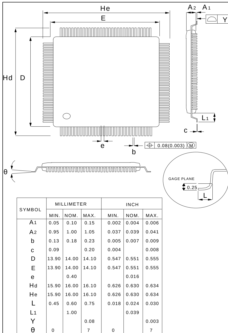
FIGURE 47 - VTQFP PACKAGE OUTLINE
