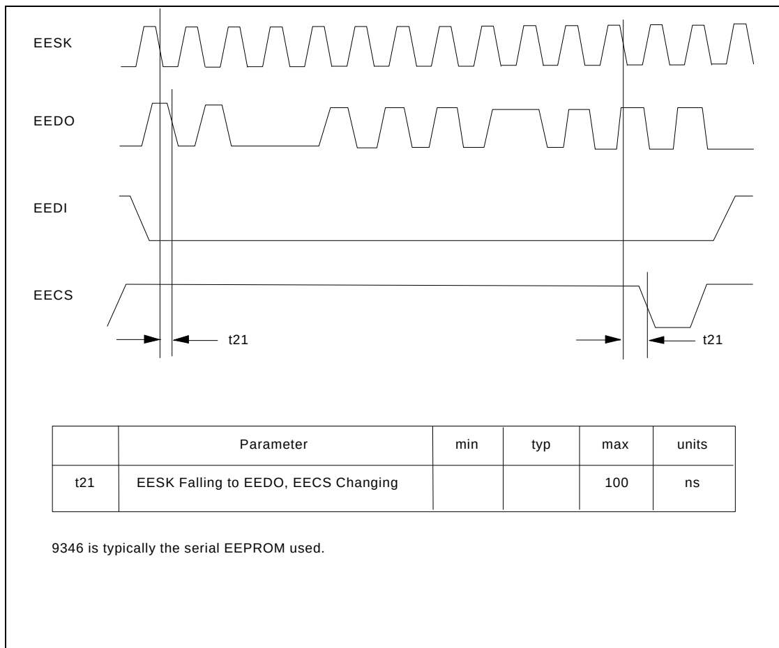
FIGURE 37 - EEPROM WRITE
