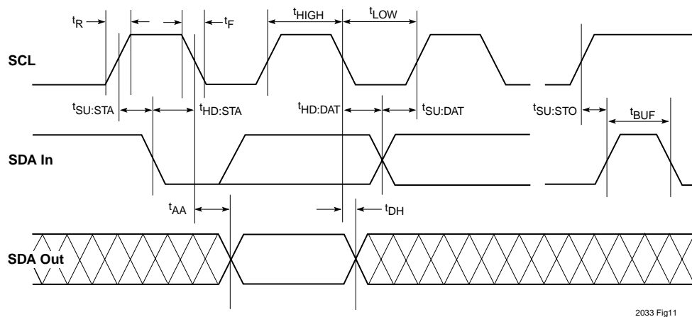
Figure 11. Interface Bus Timing
