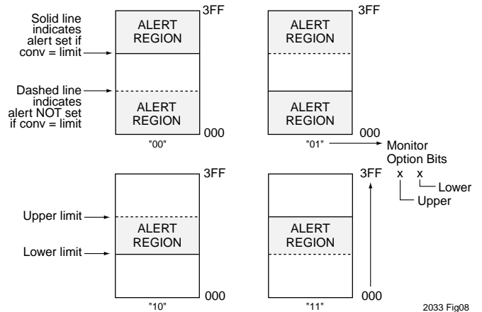
Figure 8. Four Alert Conditions
