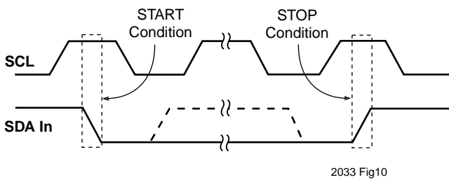
Figure 12. Start and Stop Conditions
