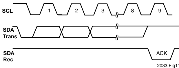
Figure 13. Acknowledge Timing
