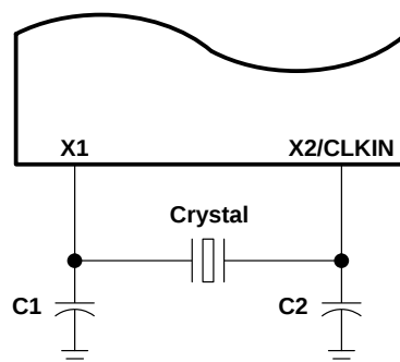
Figure 5–2. Internal Divide-by-Two Clock Option With External Crystal
