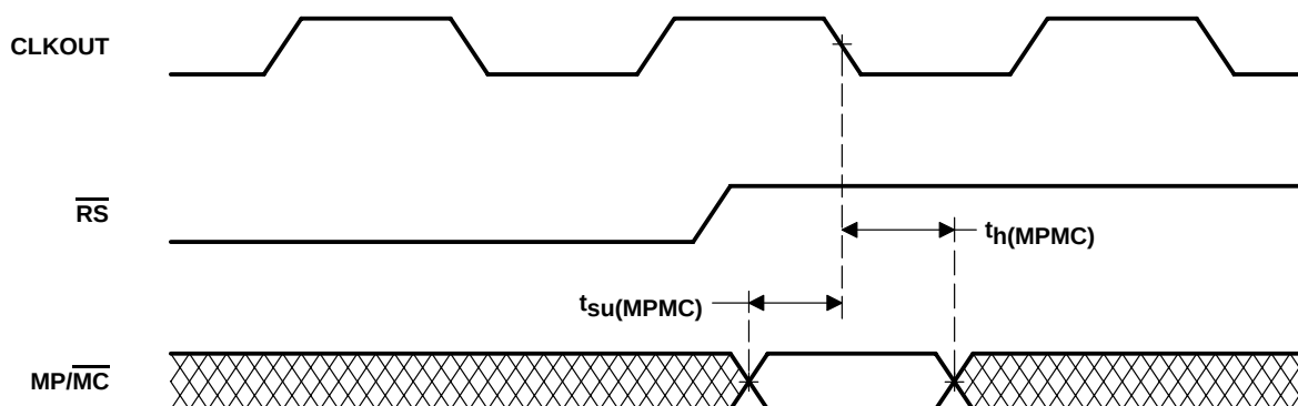
Figure 5-17. \text{MP}/\overline{\text{MC}} Timing
