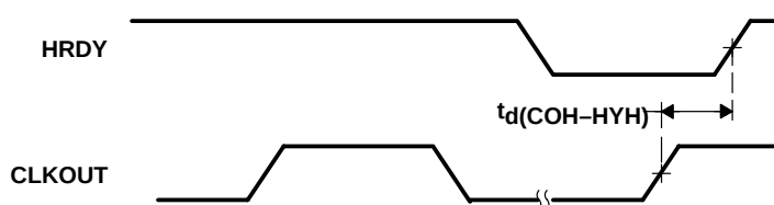
Figure 5-34. \text{HRDY} Relative to \text{CLKOUT}
