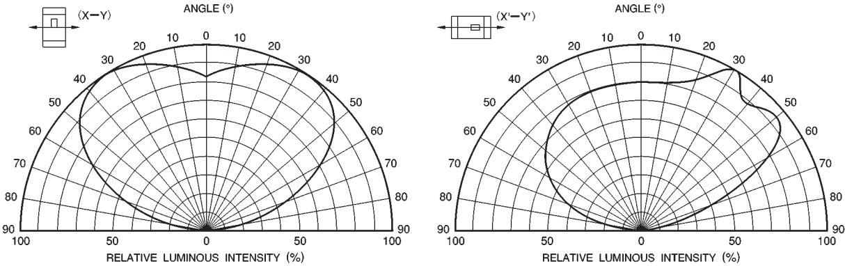
Fig. 1 Directional pattern
