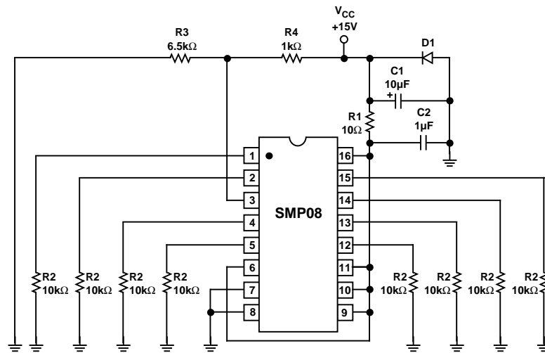
Figure 17. Burn-In Circuit
