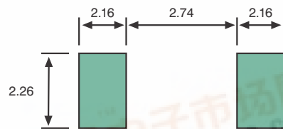
Solder Pads
