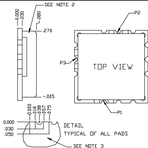
PHYSICAL DIMENSIONS
