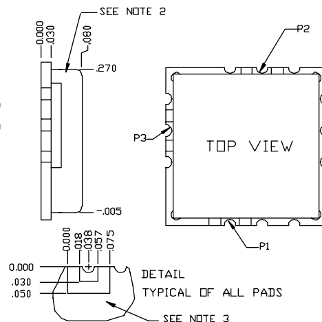
PHYSICAL DIMENSIONS
