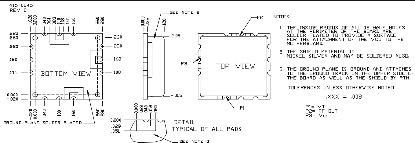
PHYSICAL DIMENSIONS
