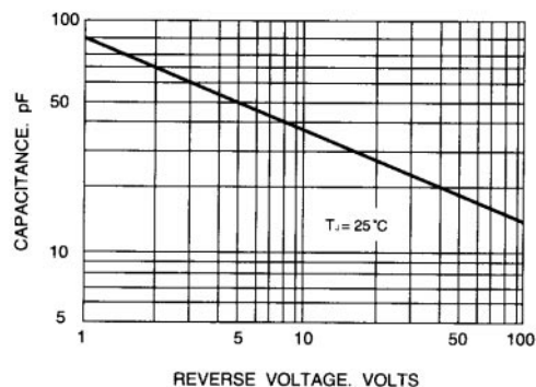
FIG. 4 - TYPICAL JUNCTION CHARACTERISTICS
