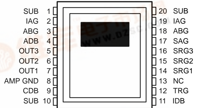
DUAL-IN-LINE PACKAGE (TOP VIEW)
