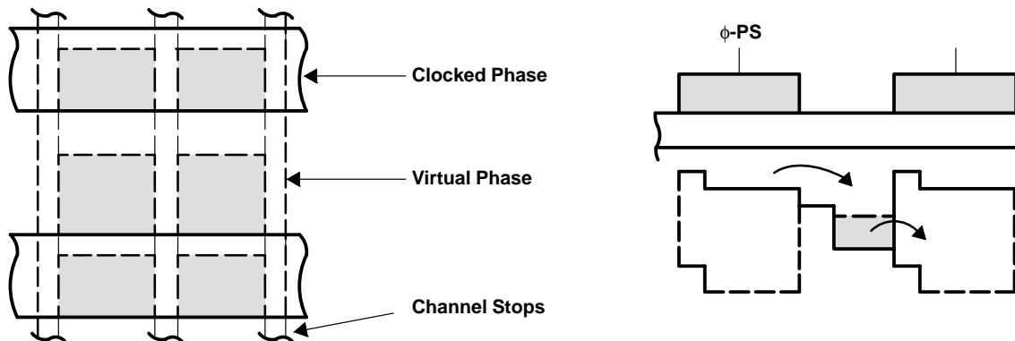
Figure 2. Charge-Transfer Process
