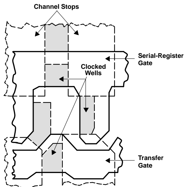
Figure 4. Interface-Region Layout
