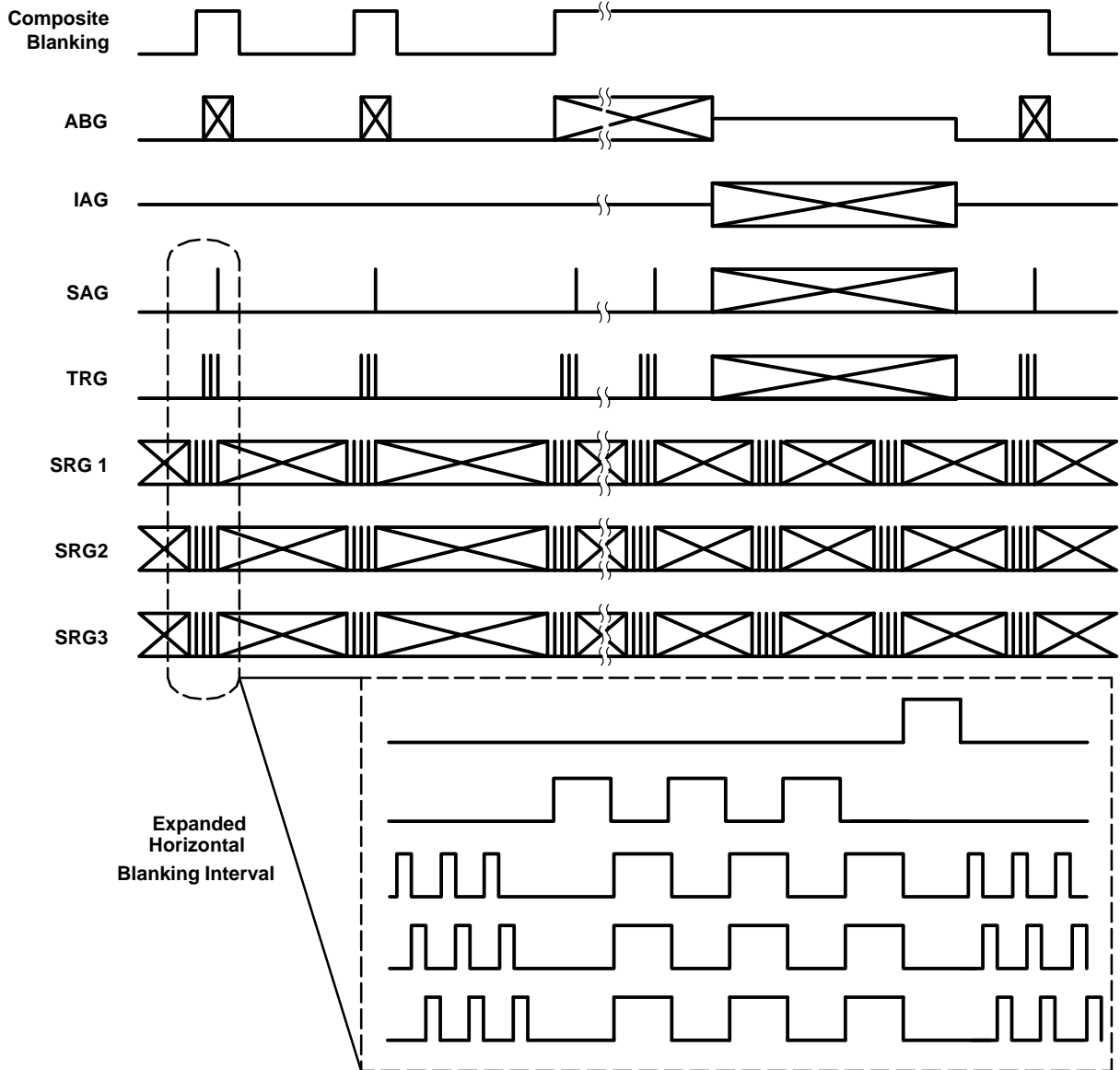
Figure 5. Timing Diagram
