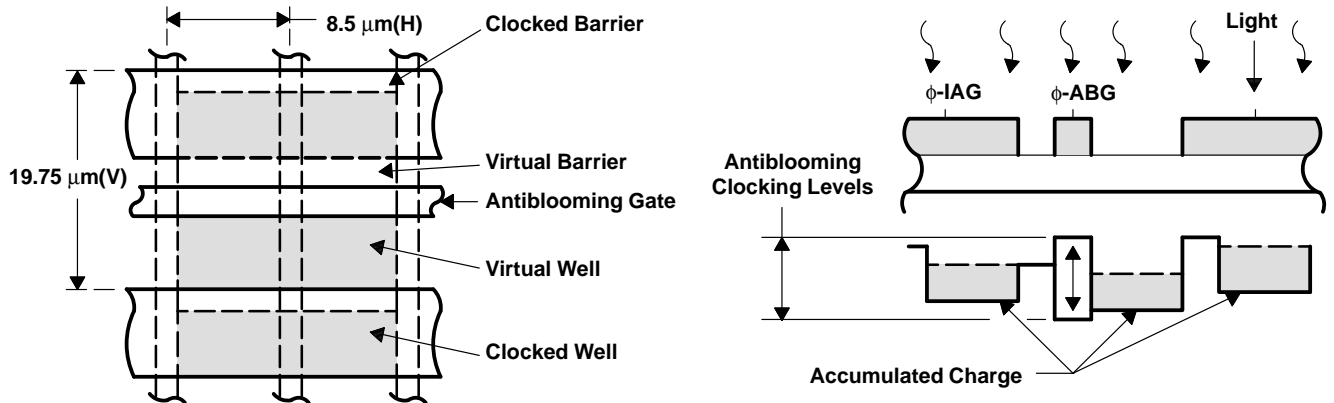
Figure 1. Charge-Accumulation Process
