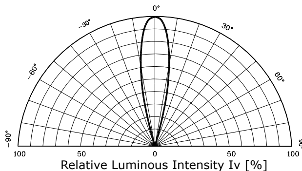
Fig. 5 Radiation Diagram
