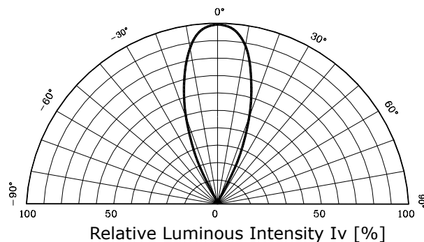
Fig. 5 Radiation Diagram
