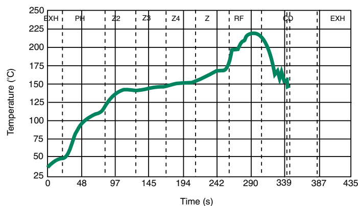
Typical Solder Reflow Thermal Profile (No-Clean Flux)
