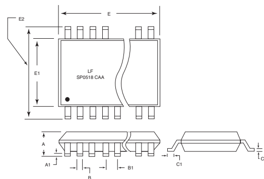
SP0518CAA - QSOP 24
