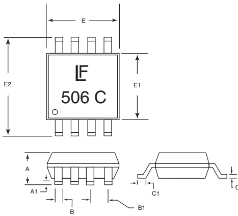
SP0506CAA - MSOP 8
