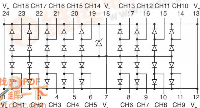
SP0518CAAT
