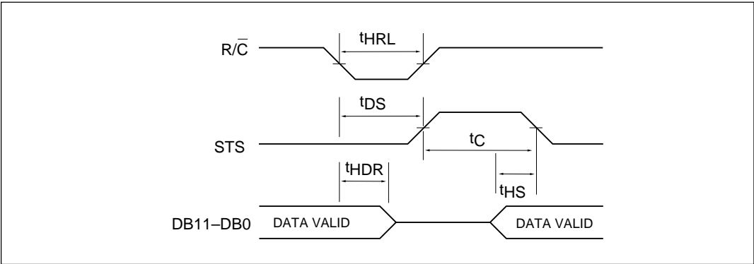
Figure 8. Low Pulse for R/C — Outputs Enabled After Conversion
