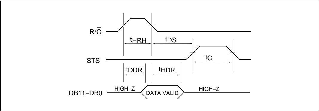
Figure 9. High Pulse For R/C — Outputs Enabled While R/C is High, Otherwise High Impedance
