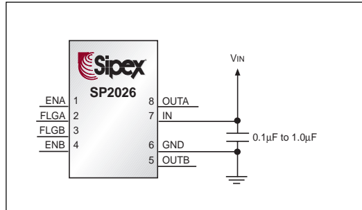
Figure 4. Bypass Capacitor at the Supply Pins
