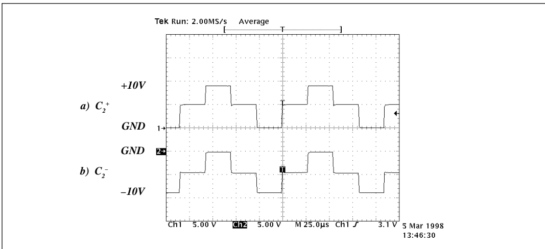
Figure 3. Charge Pump Waveform
