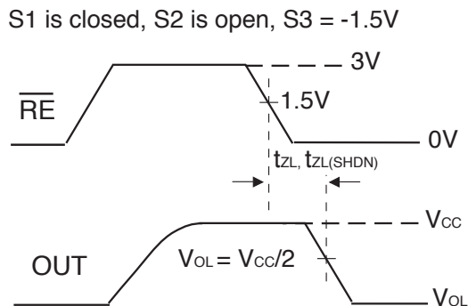
FIGURE 8. RECEIVER ENABLE & DISABLE TIMING DIAGRAM
