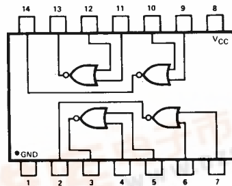
QUAD 2-INPUT
