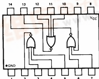
TRIPLE 3-INPUT
