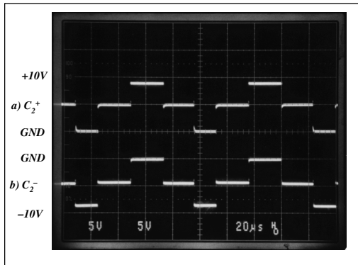
Figure 1. Charge Pump Waveforms
