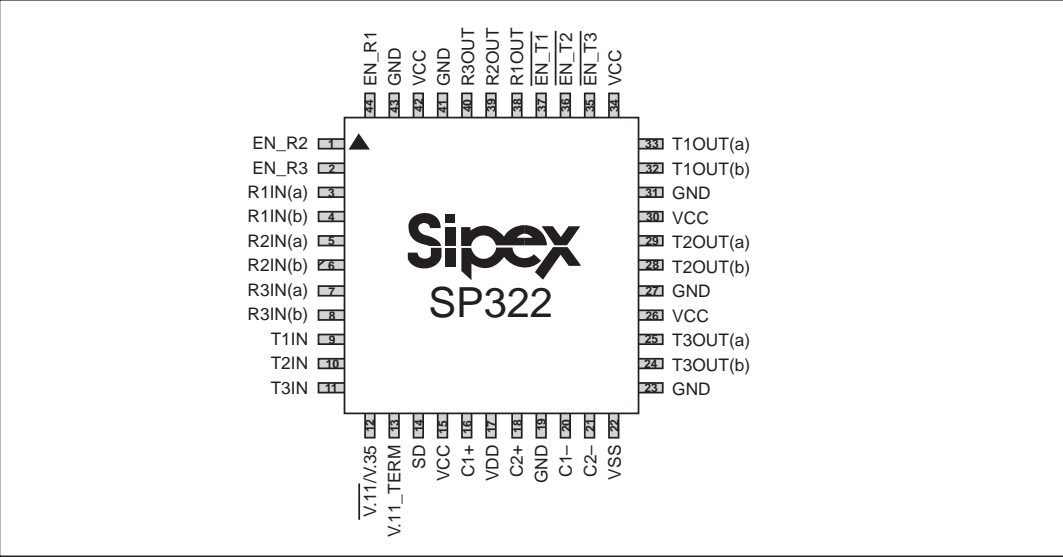
Figure 25. SP322 Pinout
