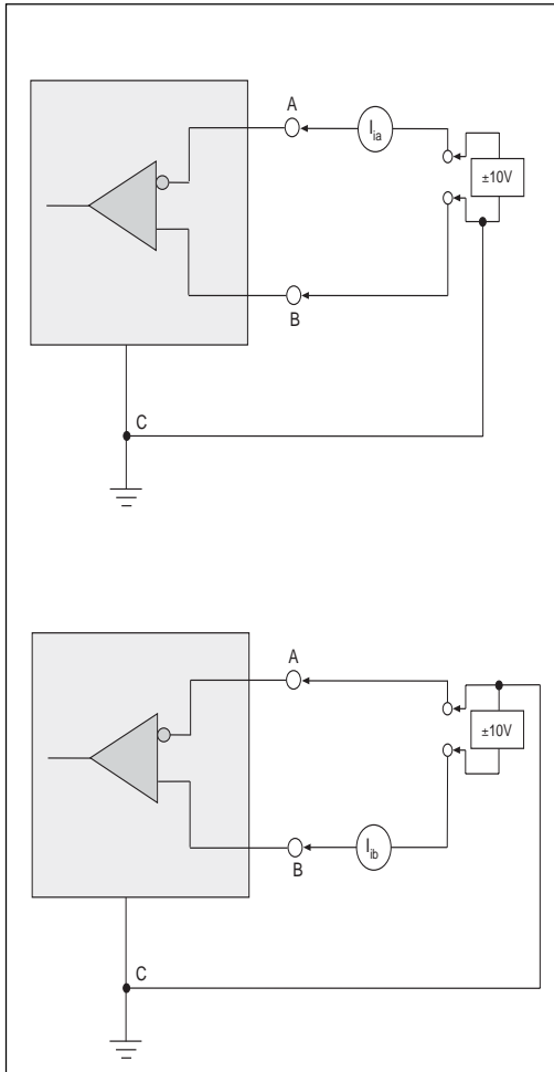
Figure 6. V.11 Receiver Input Current
