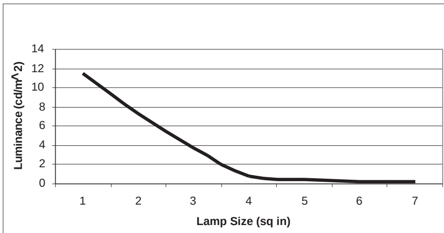
Figure 10. Luminance (candela per meter square) vs. Lamp Size
