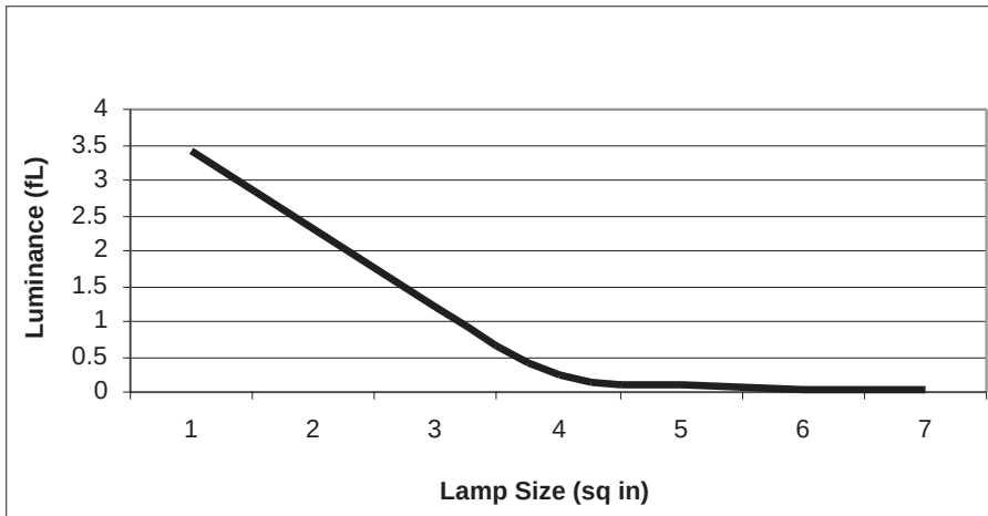
Figure 9. Luminance (Foot-Lamberts) vs. Lamp Size
