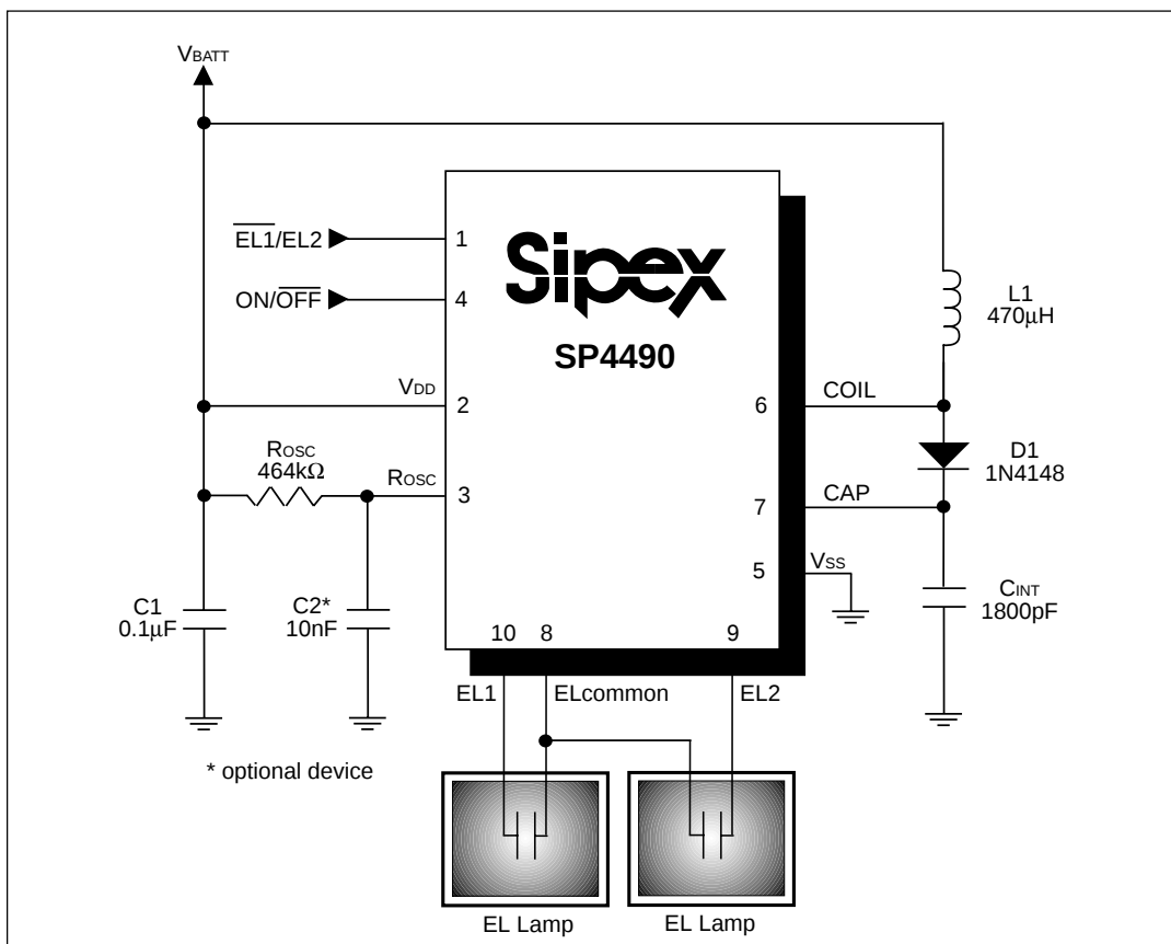
Figure 2: Typical Application Circuit of SP4490
