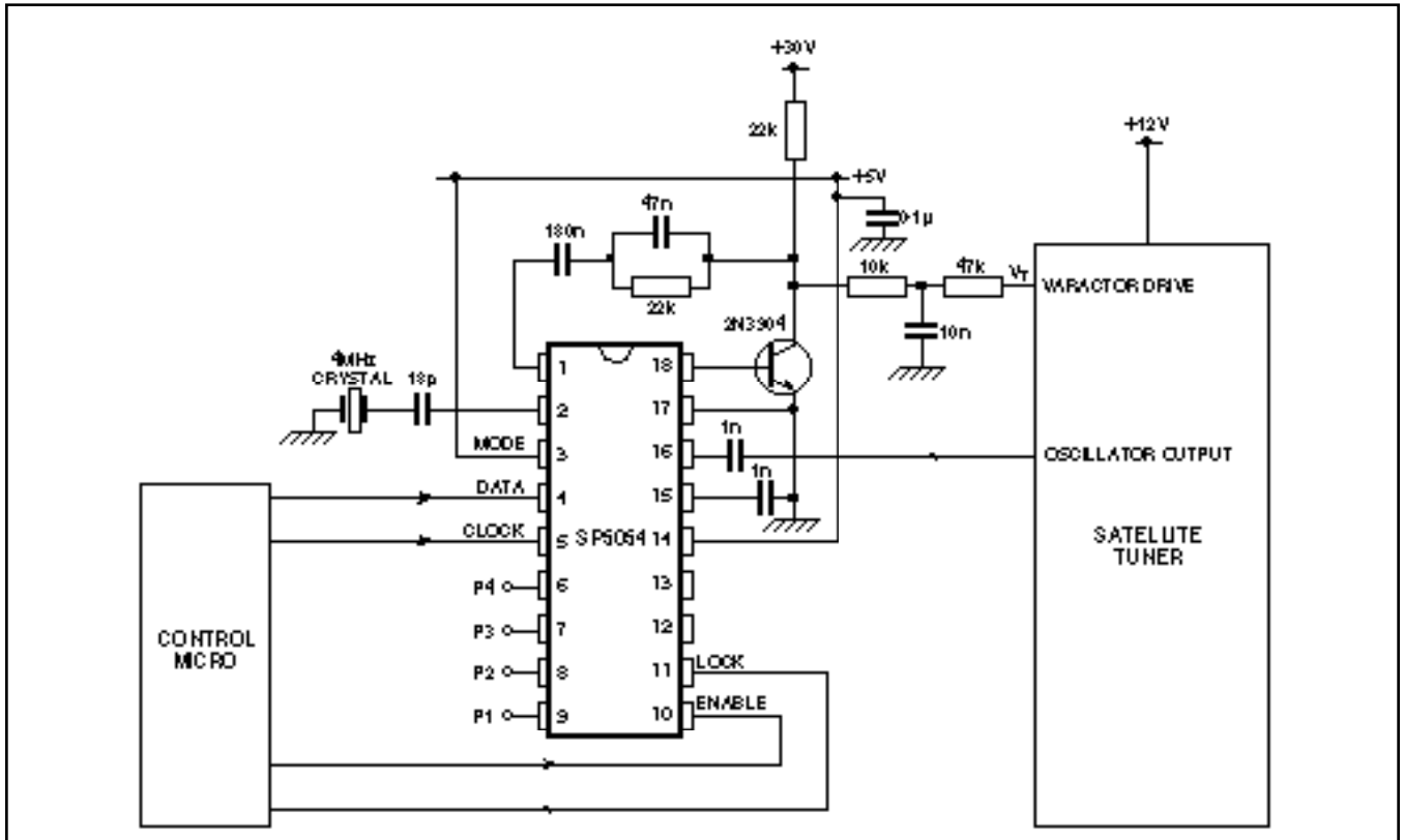
Fig. 5 Typical application ( f_{STEP} = 125\text{kHz} )
