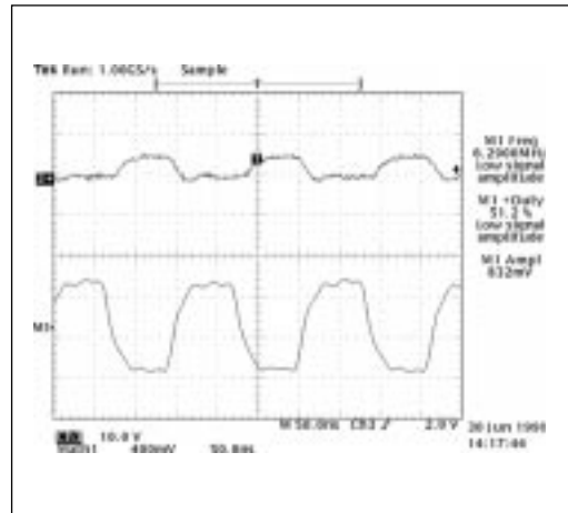
Figure 16. SP507 TxCE at 6.312MHz over 156ft.
