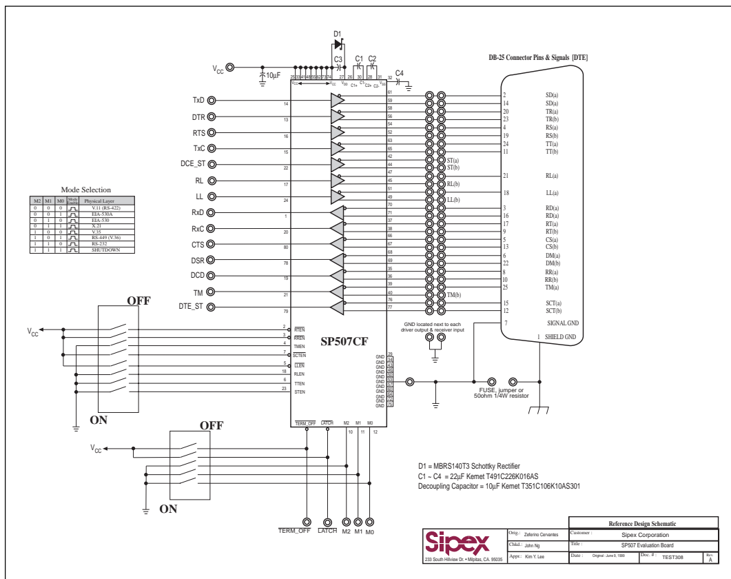
Figure 36. SP507EB Schematic
