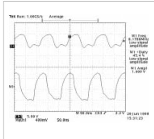
Figure 18. SP507 TxCE at 8.192MHz over 56ft.
