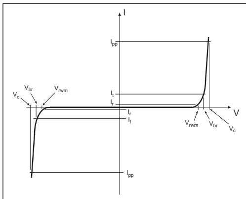
Figure 28. I-V Curve of a TVS diode
