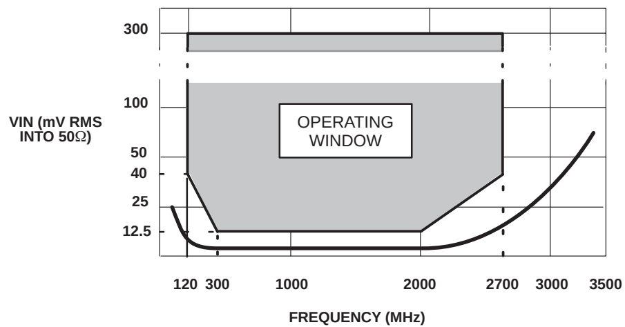
Fig. 6 Typical input sensitivity
