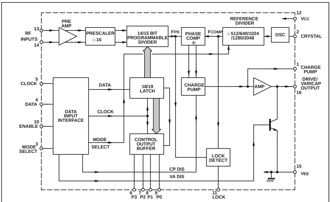
Fig. 3 Block diagram
