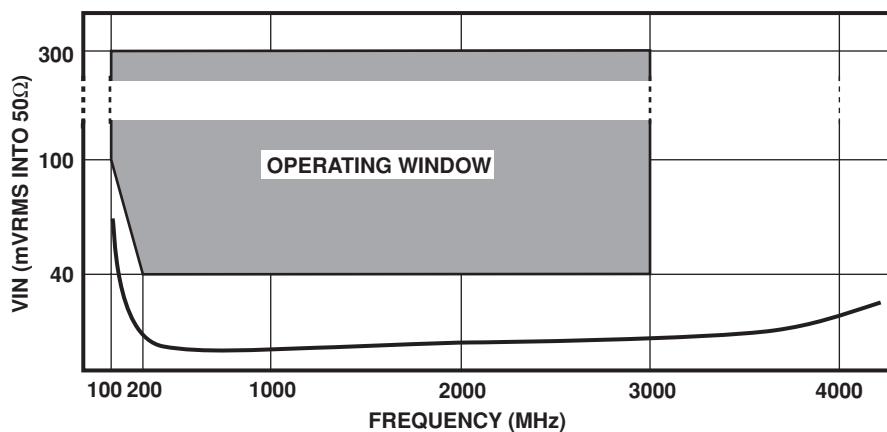
Figure 3 Typical RF input sensitivity
