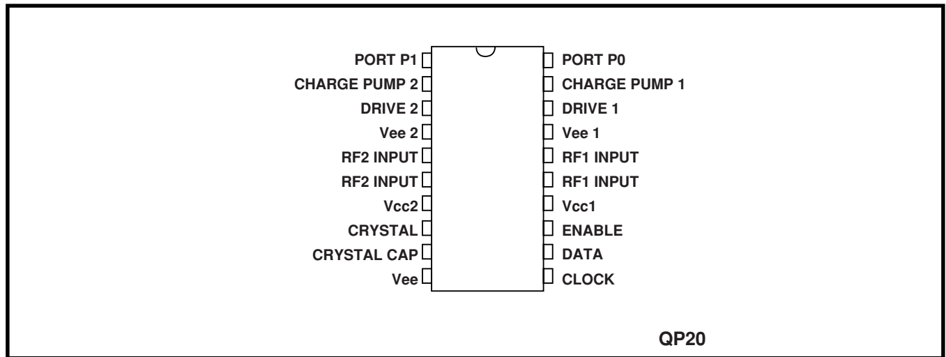
Figure 2 Pin Connections
