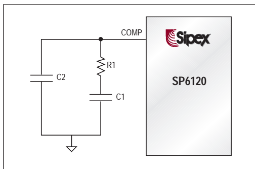
Figure 18. The RC network connected to the COMP pin
