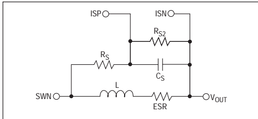
Figure 20: Current Sensing
