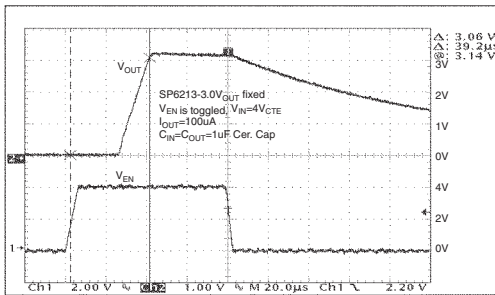
Turn-on Characteristic ( V_{IN} = 4V , I_{OUT} = 100\mu A )
