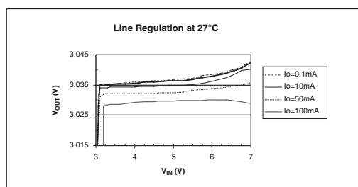
Output Voltage vs. Input Voltage
