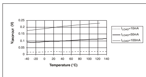
Dropout Voltage vs. Temperature
