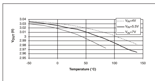
Output Voltage vs. Temperature ( I_{OUT} = 100mA )
