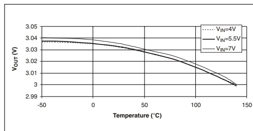
Output Voltage vs. Temperature ( I_{OUT} = 10mA )
