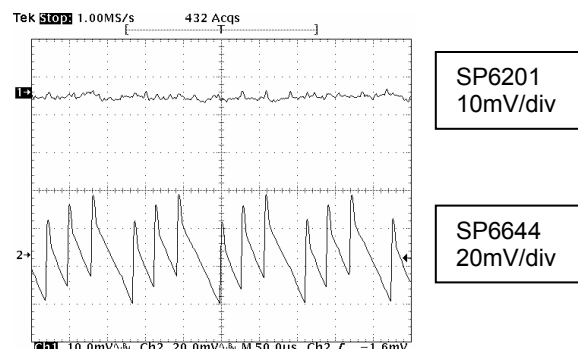
Figure 8. SP6644 and SP6201 Output Ripple Rlim=2.5K (Vin = 1.3V, Vout = 3.3V, Iout=80mA)
