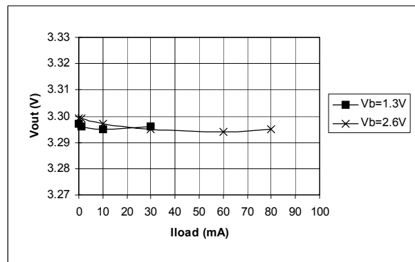
Figure 4. Line/Load Rejection Vs Output Current (Vout = 3.3V) Rlim=5K
