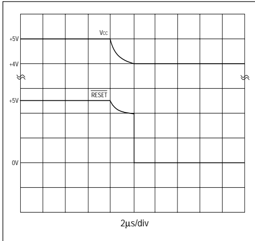
Figure 4A. SP703 RESET Response Time
