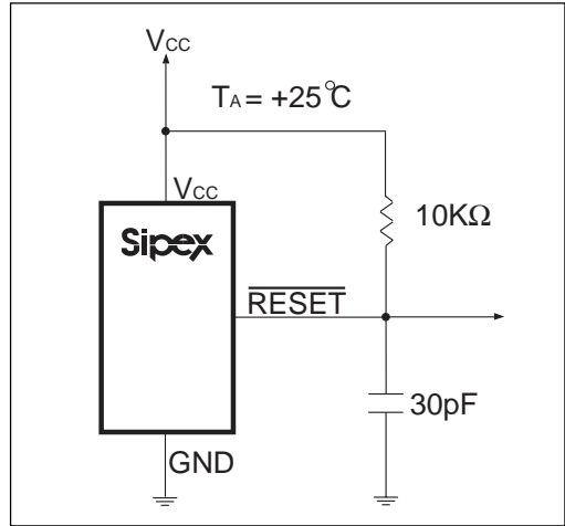
Figure 4B. Circuit for the RESET Response Time
