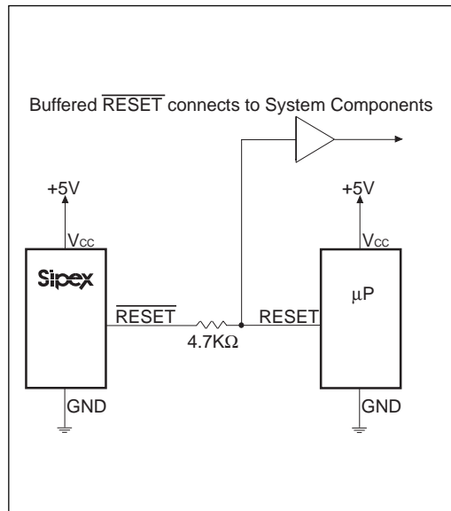
Figure 19. Interfacing to Microprocessors with Bidirectional \overline{\text{RESET}} I/O for the SP705/706/707/708
