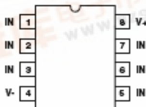
SP721 (PDIP, SOIC) TOP VIEW
