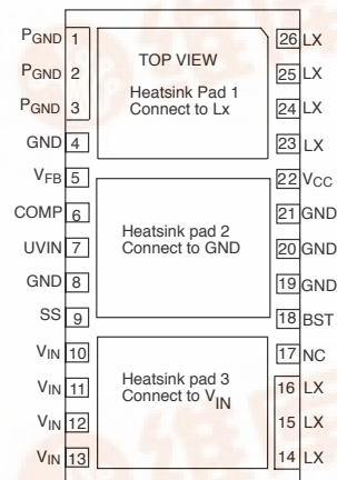
SP7655 DFN PACKAGE 7mm x 4mm
