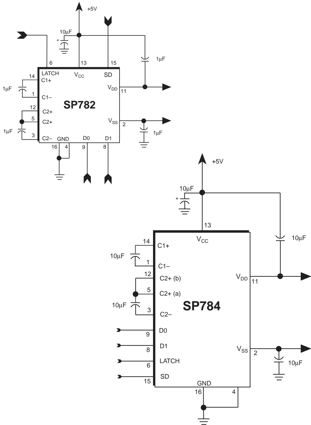
Figure 9. SP782 and SP784 Block Diagrams
