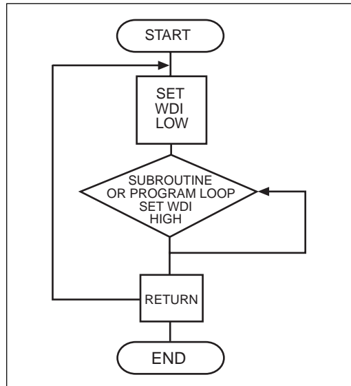
Figure 16. Watchdog Flow Diagram
