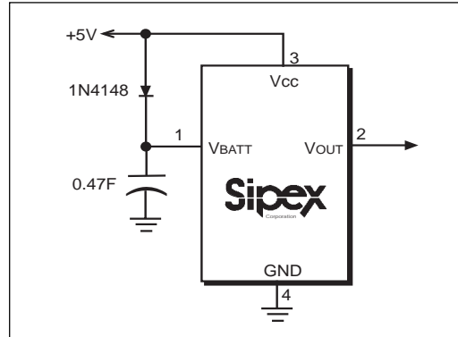
Figure 12. High Capacity Capacitor on V_{BATT}
