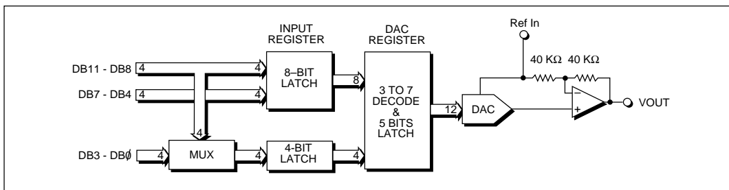
Figure 1. Detailed Block Diagram (only one DAC shown)
