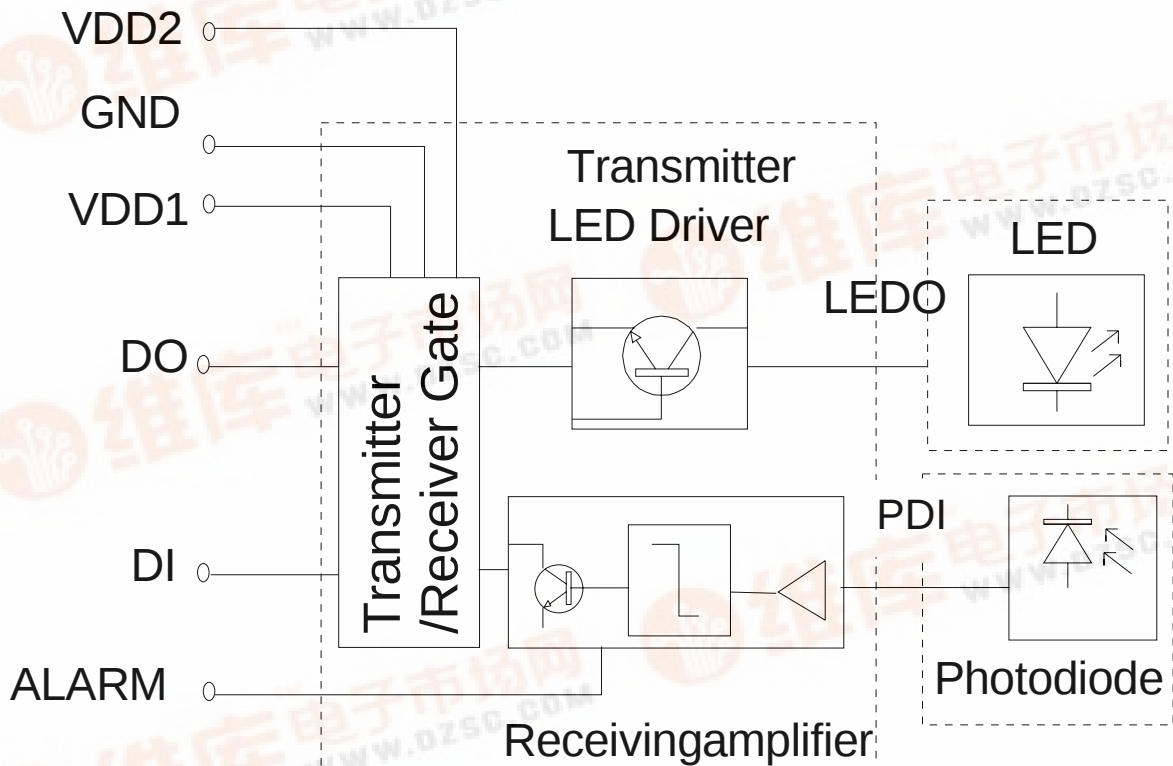
Fig. 1: Basic functional units of SPF BFT3 02
