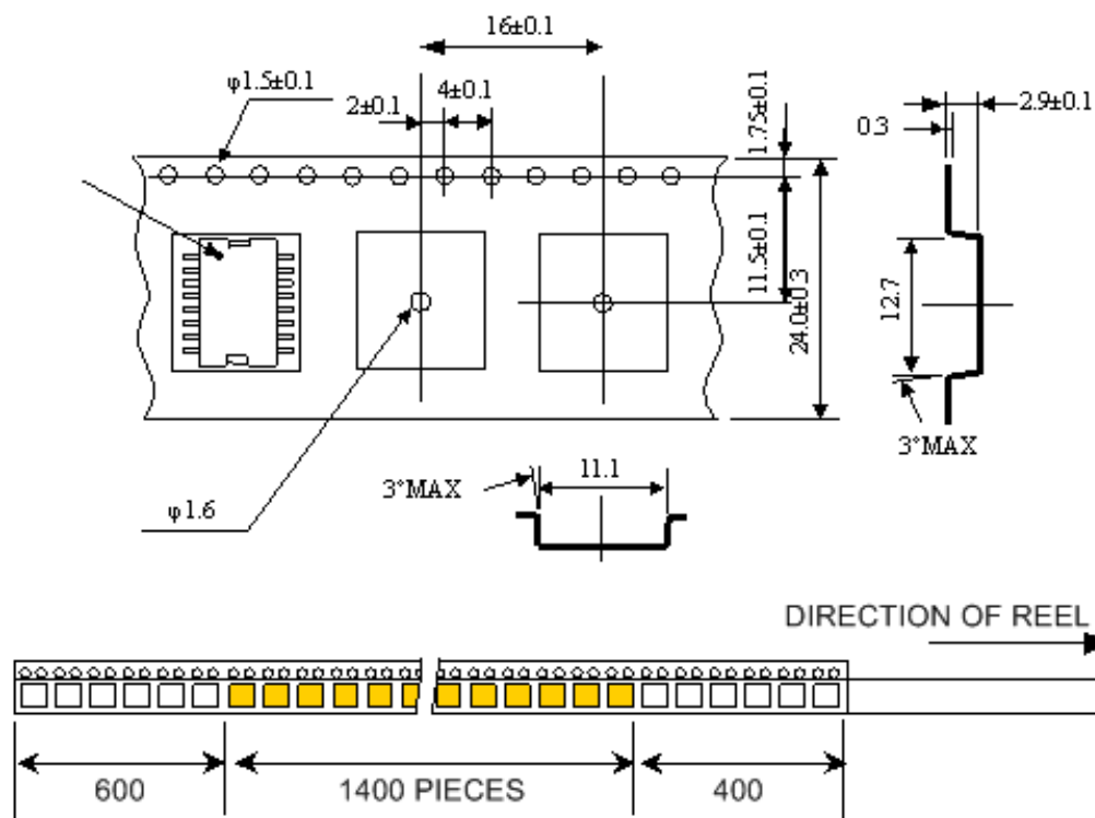
Tape and Reel Dimensions in Millimeters
