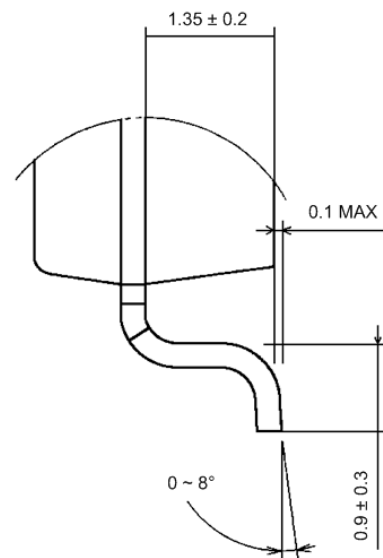
View A
