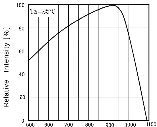
Fig.5 Spectrum Sensitivity
